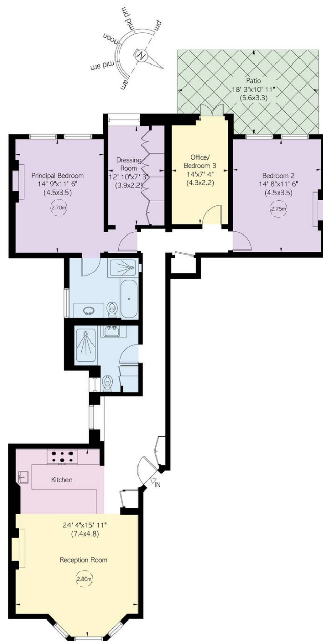
Ground Floor
