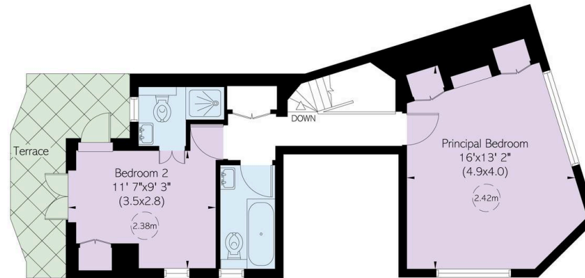
Third Floor
